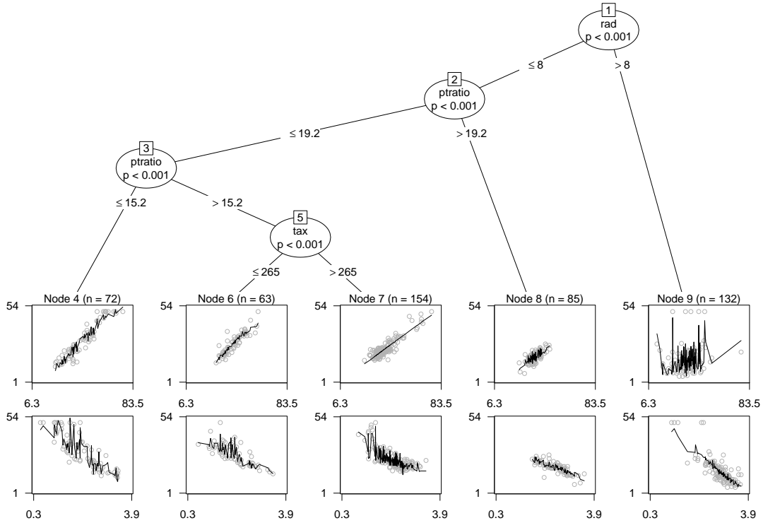
Figure 1: Linear-regression-based tree for the Boston housing data. The plots in the leaves give partial scatter plots for (rm)^2 (upper panel) and \log(lstat) (lower panel).
