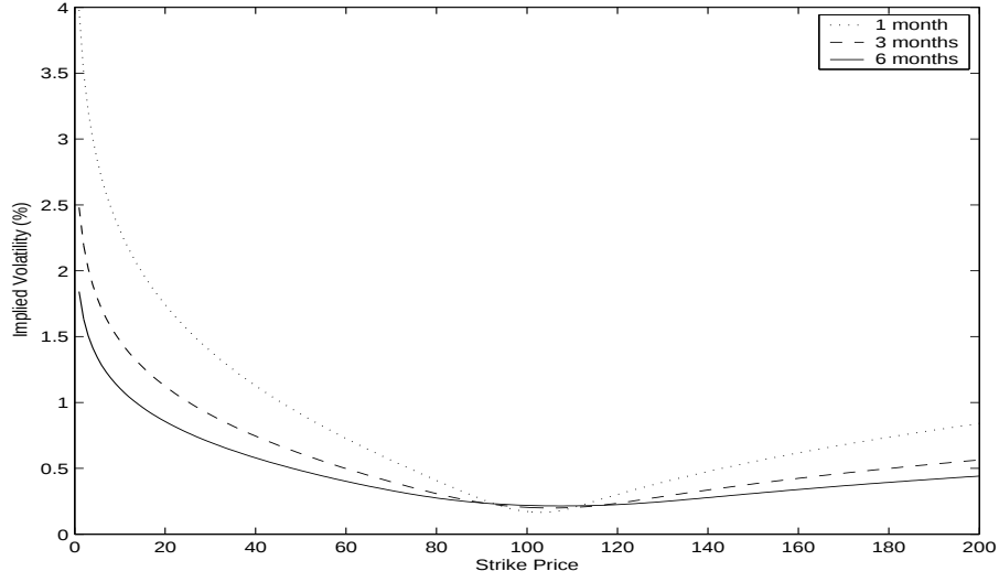
Figure 6: Black-Scholes implied volatility for the Lévy-Stable call option prices when returns follow a symmetric Lévy-Stable motion with \alpha = 1.7 , \sigma_{LS} = 0.7673 and \sigma_\ell = 0.1401 and three expiry dates: one, three and six months.
