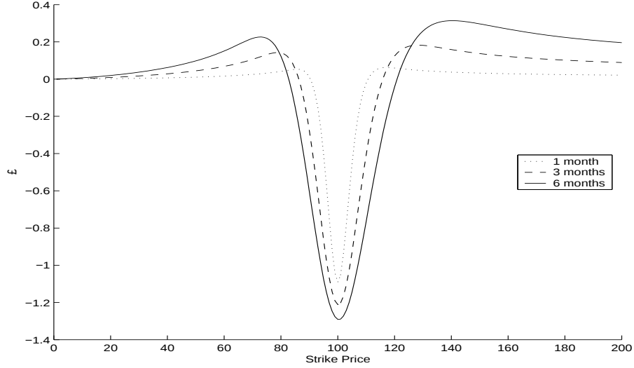
Figure 3: Difference between Lévy-Stable and Black-Scholes Call option prices for different expiry dates: one, three and six months. In the Black-Scholes annual volatility is \sigma_{BS} = 20\% .
