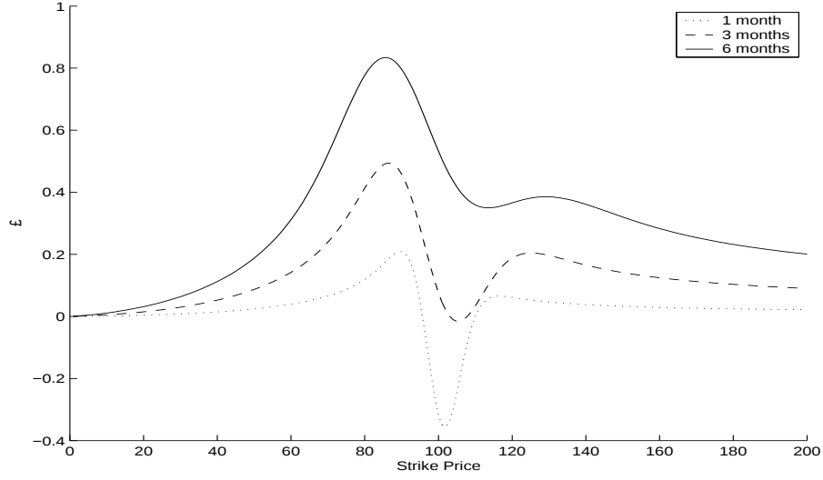
Figure 5: Difference between Lévy-Stable and Black-Scholes call option prices for different expiry dates: one, three and six months. In the Black-Scholes annual volatility is \sigma_{BS} = 0.20 and in the asymmetric Lévy-Stable case the scaling parameters are \sigma_{LS} = 0.7673 and \sigma_\ell = 0.1401 .
