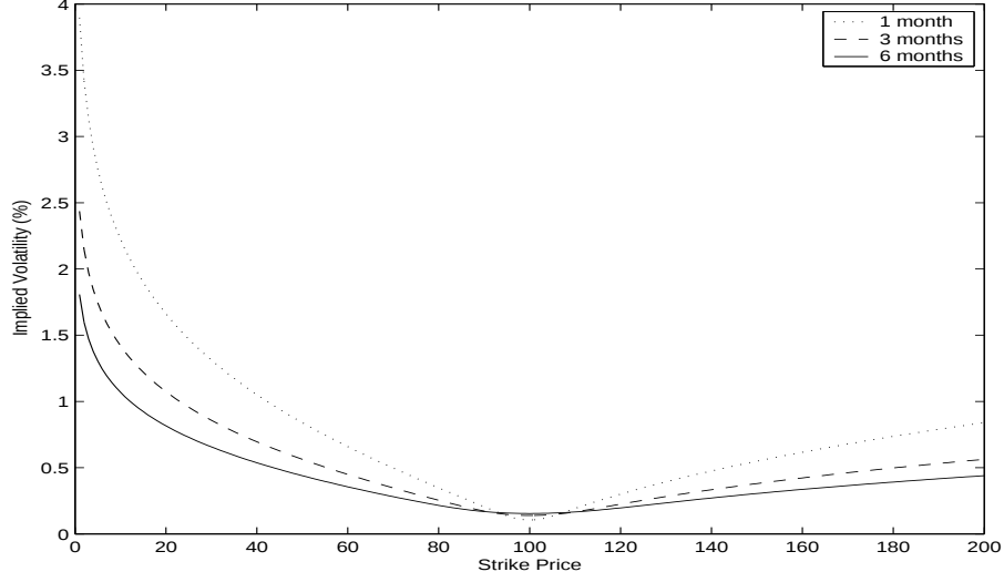
Figure 4: Black-Scholes implied volatility for the Lévy-Stable Call option prices when returns follow a symmetric Lévy-Stable motion with \alpha = 1.7 , \beta = 0 and three expiry dates: one, three and six months.
