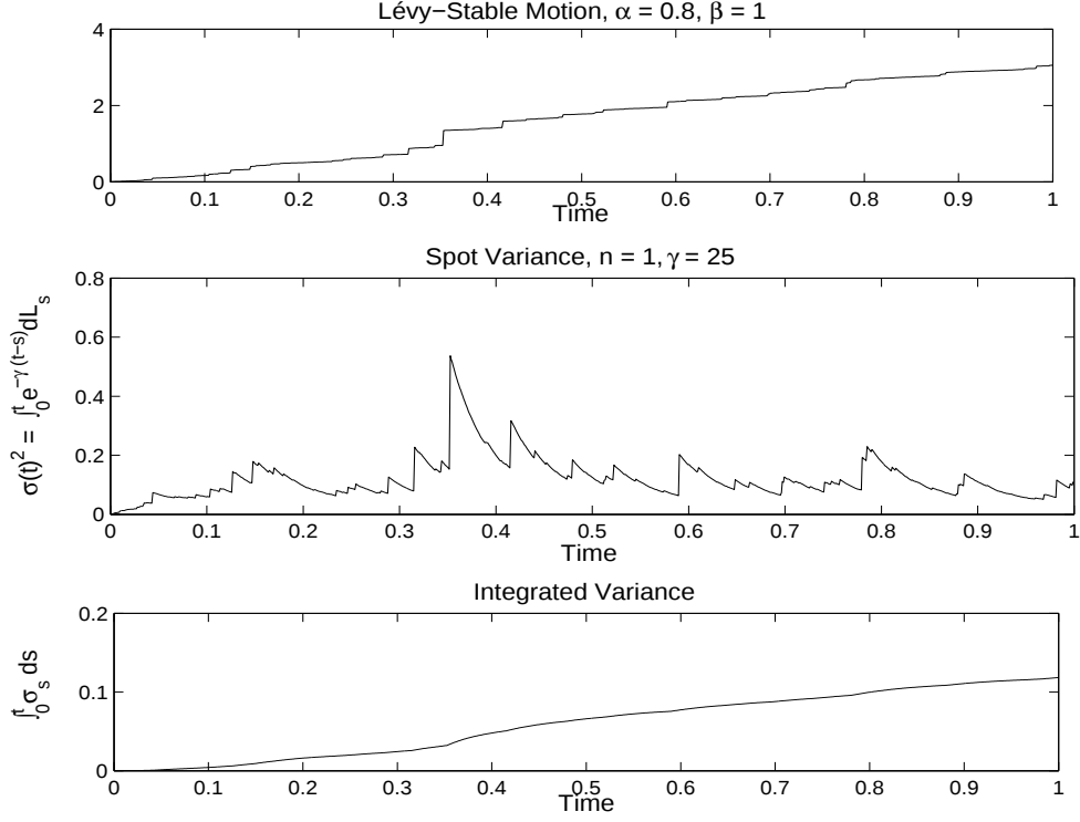
Figure 1: Simulated integrated variance with kernel g(T-s) = 25^{-1} (1 - e^{-25(1-s)}) .
